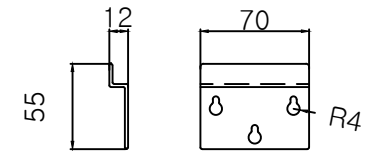
Wall Bracket
