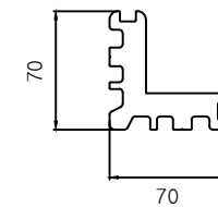
Corner Bracket
