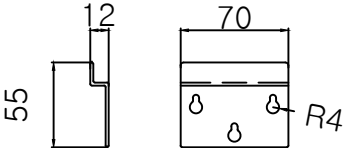
Wall Bracket
