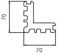
Corner Bracket
