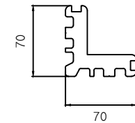
Corner Bracket
