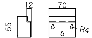
Wall Bracket
