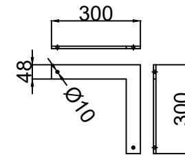
Conner Bracket
