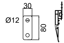
Wall Bracket
