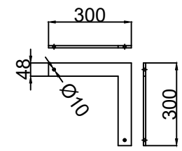
Conner Bracket
