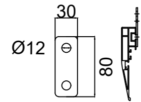
Wall Bracket
