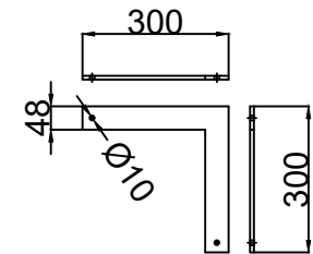
Conner Bracket
