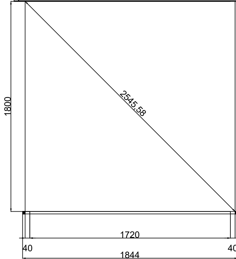
Front View
