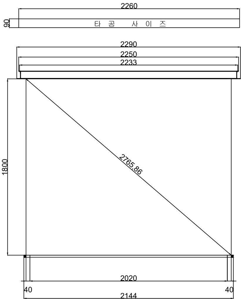
Front View
