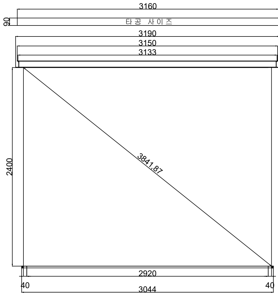
Front View
