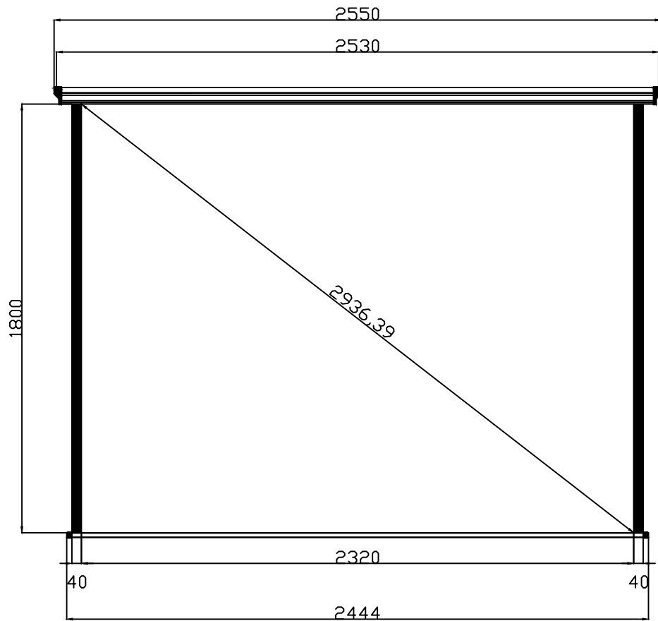
Front View
