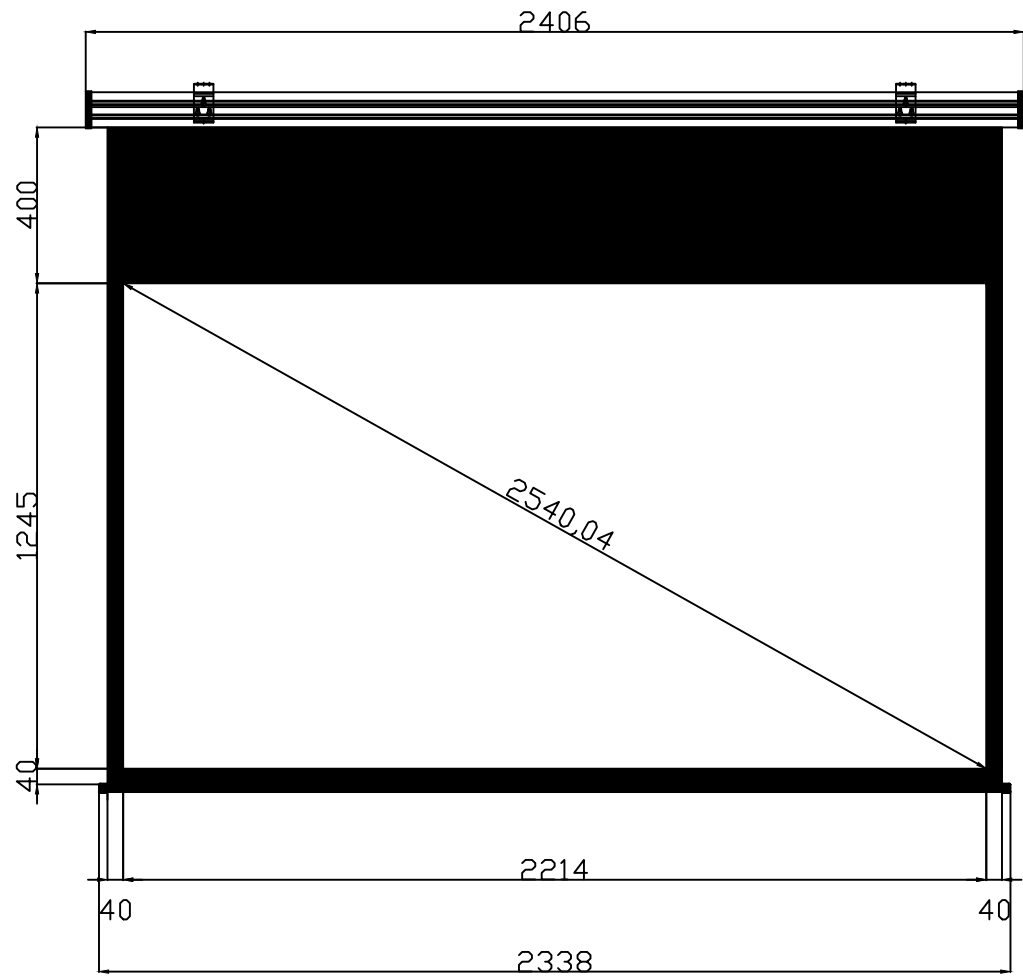
Front View
