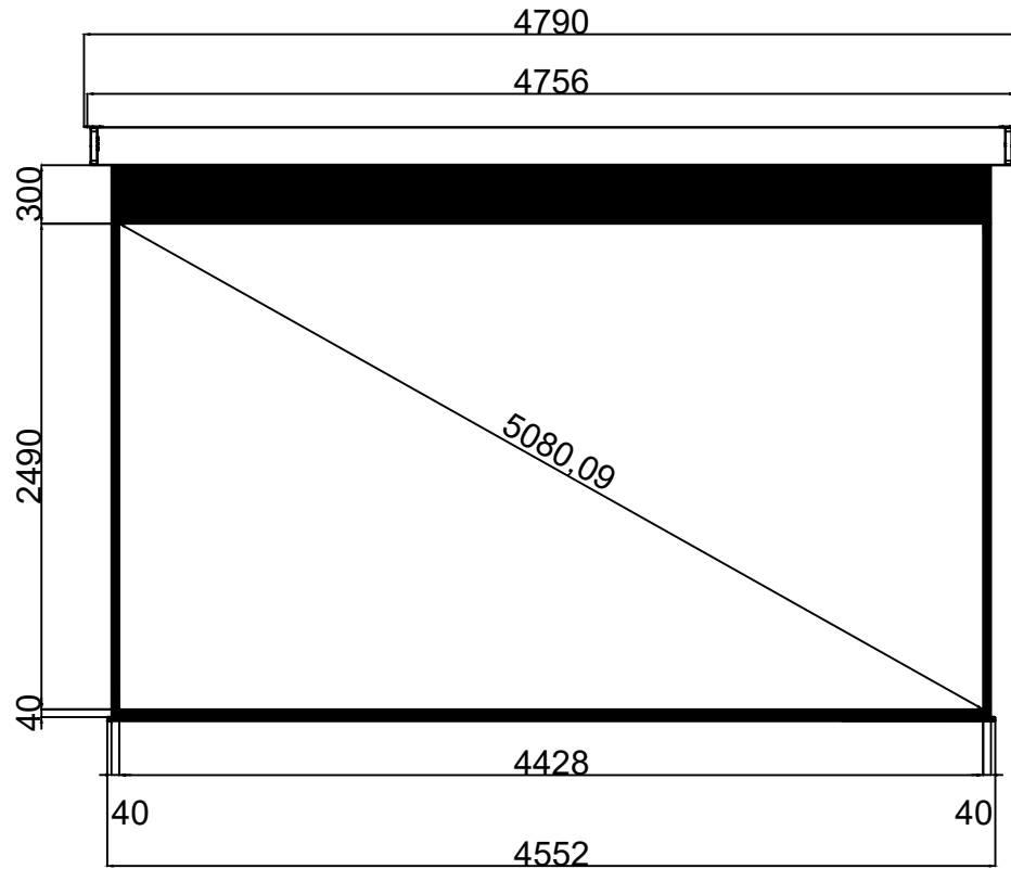
Front View
