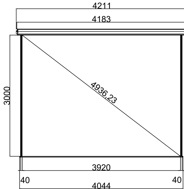
Front View
