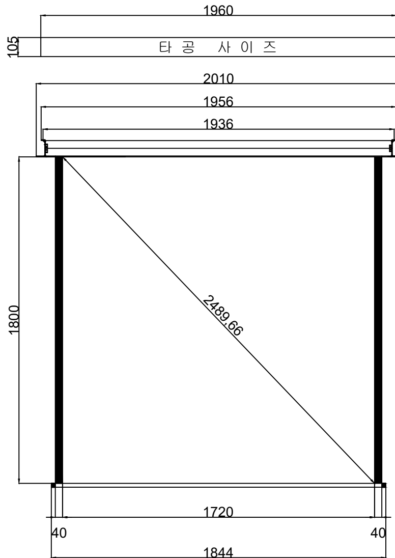
Front View
